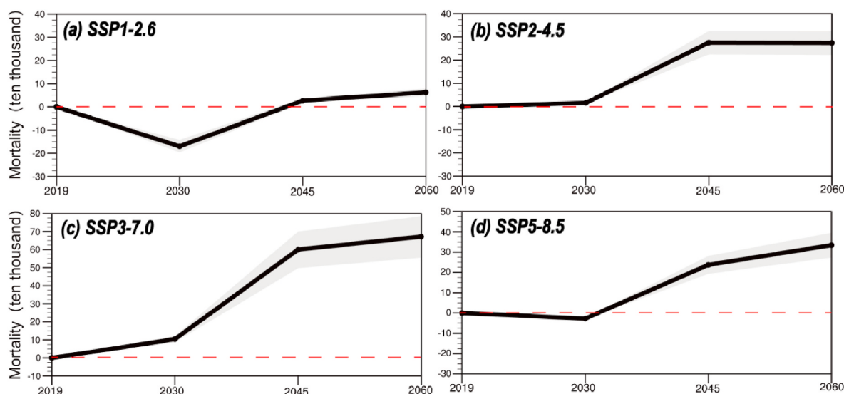
Fig. 6. Future changes in premature mortalities attributable to PM_{2.5} exposure in years of 2030, 2045 and 2060 relative to 2019 under different SSP scenarios: (a) SSP1-2.6, (b) SSP2-4.5, (c) SSP3-7.0, and (d) SSP5-8.5. The black dotted line is the ensemble mean averaged from four CMIP6 models, and the gray shaded areas represent the 95% confidence interval. SSP1-2.6, SSP2-4.5, SSP3-7.0 and SSP5-8.5 represent sustainable development scenario, middle of the road scenario, regional rivalry scenario, and fossil fuel-driven development scenario, respectively.
