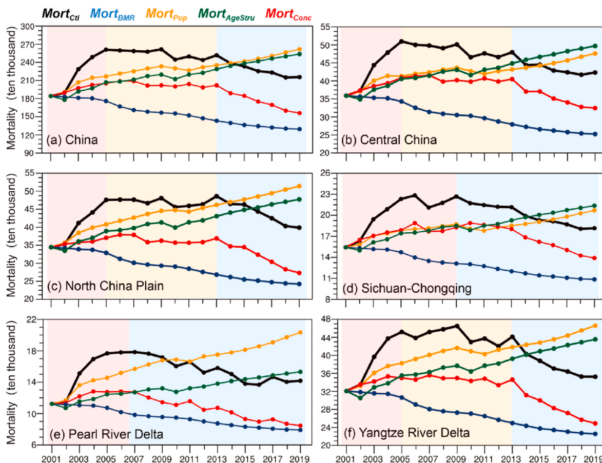
Fig. 7. Yearly premature mortalities attributable to long-term PM_{2.5} exposure during 2001–2019 in normal-condition experiment and the four sensitivity experiments averaged over (a) China, (b) Central China, (c) North China Plain, (d) Sichuan-Chongqing region, (e) Pearl River Delta, and (f) Yangtze River Delta. The light red (yellow, blue) background indicates a phase of continuous increase (fluctuating, decrease) in premature deaths according to the normal-condition experiment.
