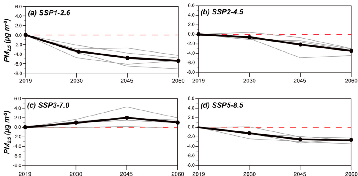
Fig. 2. Future changes in PM 2.5 concentrations in years of 2030, 2045 and 2060 relative to 2019 under different SSP scenarios: (a) SSP1-2.6, (b) SSP2-4.5, (c) SSP3-7.0, and (d) SSP5-8.5. The gray lines represent the simulated values from the four CMIP6 models, and the black dotted line is the ensemble mean. SSP1-2.6, SSP2-4.5, SSP3-7.0 and SSP5-8.5 represent sustainable development scenario, middle of the road scenario, regional rivalry scenario, and fossil fuel-driven development scenario, respectively.
