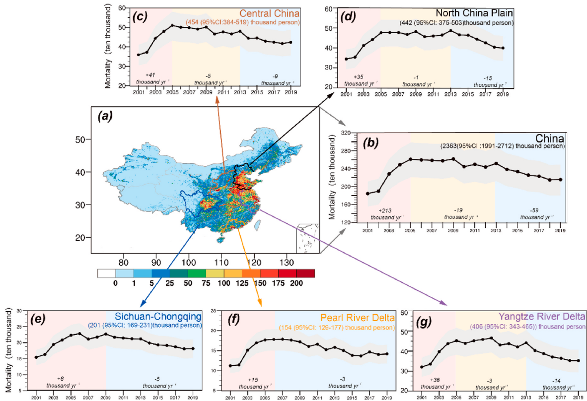
Fig. 5. Spatial-temporal distribution characteristics of premature deaths caused by long-term exposure to PM 2.5 in China during 2001–2019. (a) Spatial distribution of 19-year-mean premature deaths. (b–g) Annual mean premature deaths (black dotted line) averaged over China and the five key regions (Central China, North China Plain, Sichuan-Chongqing region, Pearl River Delta, and Yangtze River Delta) during 2001–2019. The gray shaded areas represent the 95% confidence interval. The light red (yellow, blue) background indicates a phase of continuous increase (fluctuating, decrease) in premature deaths. Mean premature deaths averaged over 2001–2019 and the trends in each time period are also shown in each panel.
